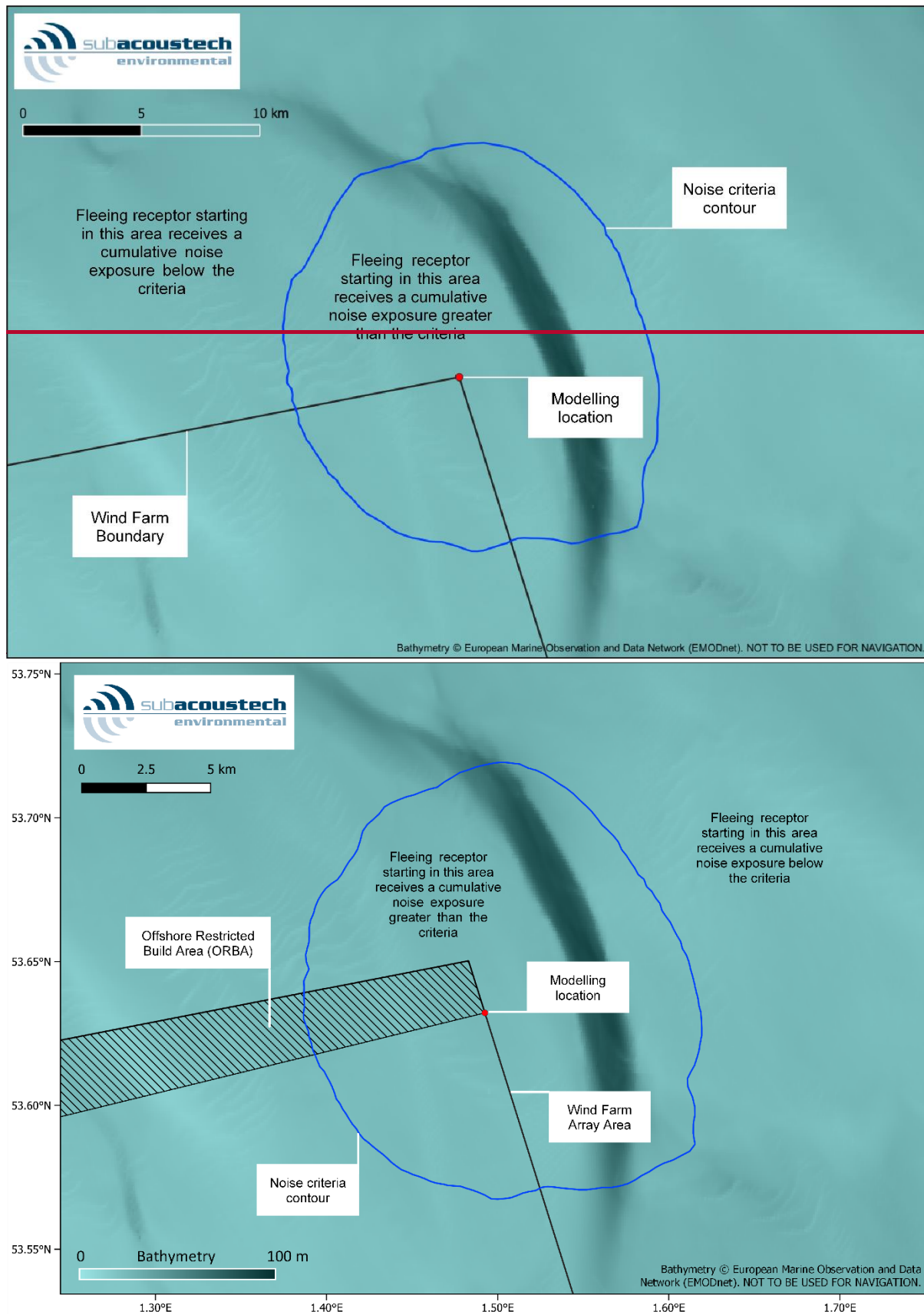
Figure 3-6 Plot showing a fleeing animal SEL_{cum} criteria contour and the areas where the cumulative noise exposure will exceed the impact criteria
