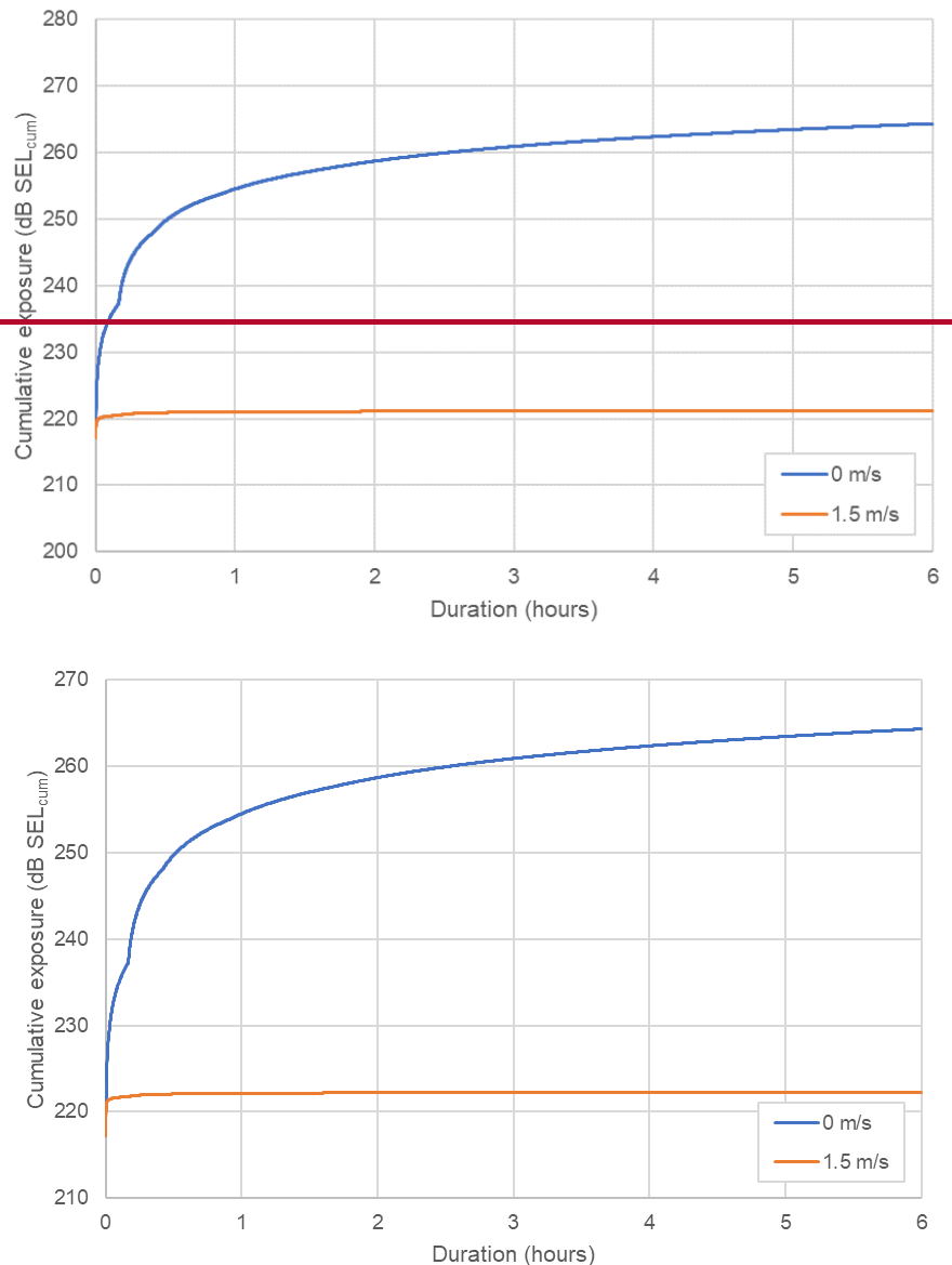
Figure 3-5 Cumulative received noise levels (SEL cum ) for receptors during monopile foundation parameters at the NE location, assuming both a stationary and fleeing receptor starting at a location 1 m from the noise source
